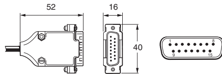
15 pin D type plug (Termination code D, L)
