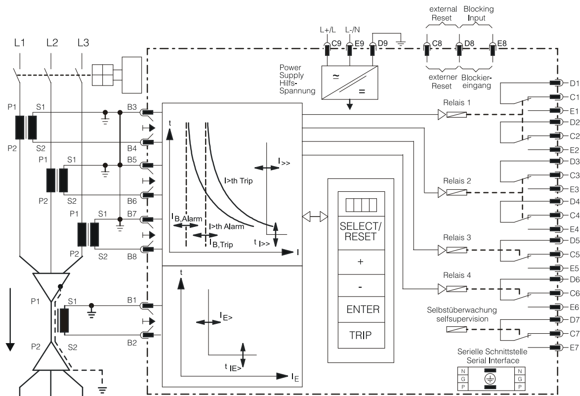
Figure 3.1: Connection diagram
