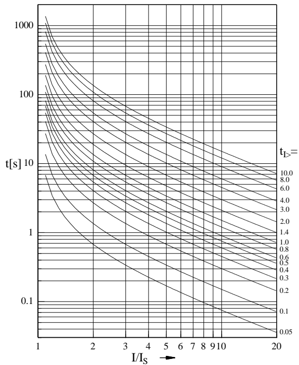
Figure 7.3: Very Inverse
