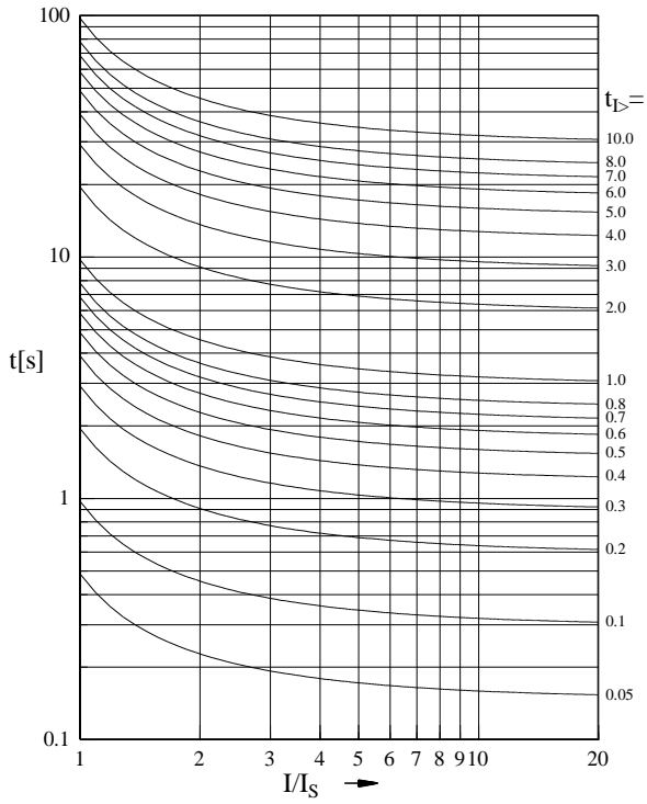
Figure 7.8: RI-Inverse
