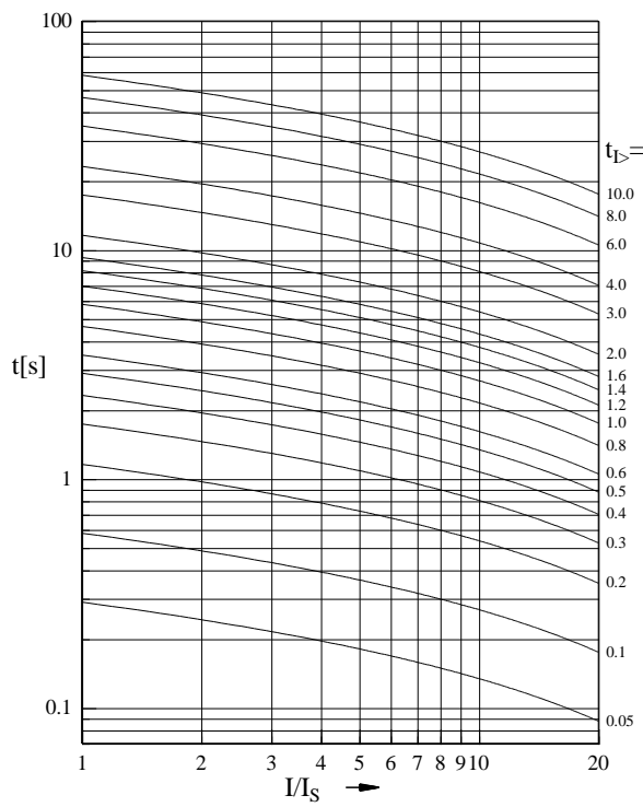
Figure 7.7: RXIDG-characteristic
