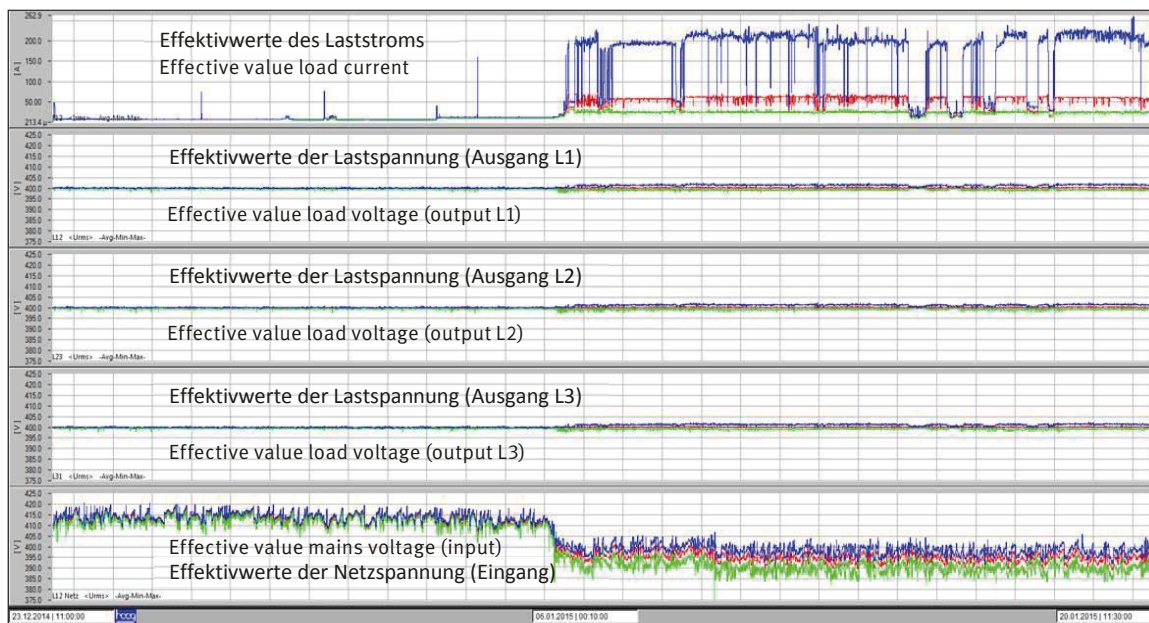
Recording of load current as well as output and input voltage. The red line shows the 10 minute mid-vale, the blue line the maximum peak value and the green line the minimal peak value.
