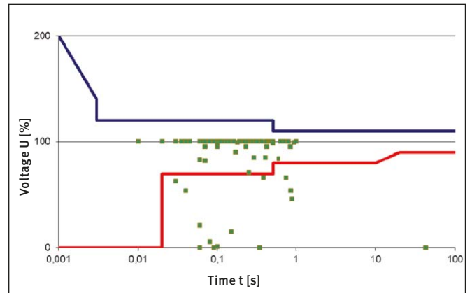
Interference ratio with OLIVER
