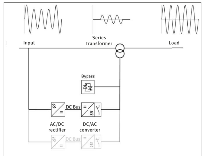
OLIVER principle of function
