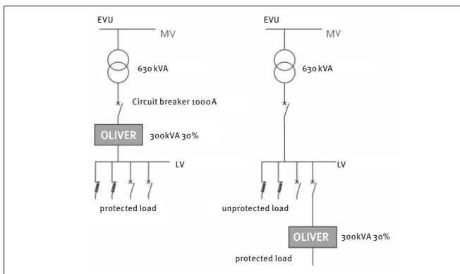
Main security with OLIVER
