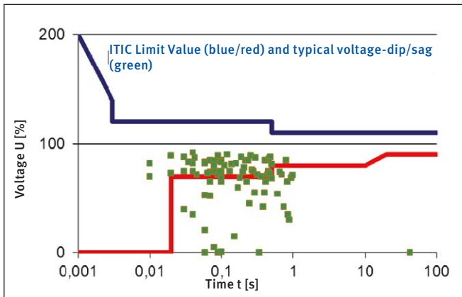
Interference ratio without OLIVER
