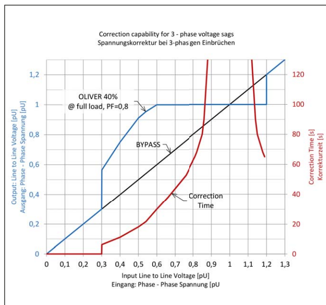
Correction values for 3-phase voltage-dips/sag
