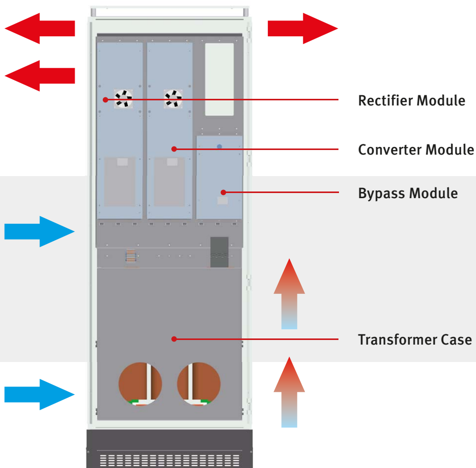
Climate concept and structure of OLIVER cabinet system
