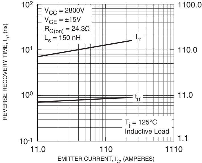
FREE-WHEEL DIODE REVERSE RECOVERY CHARACTERISTICS (TYPICAL)
