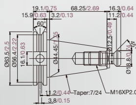
CAT40
