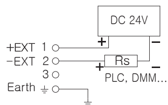
4~20mA Current out
