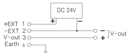
1~5V Voltage out
