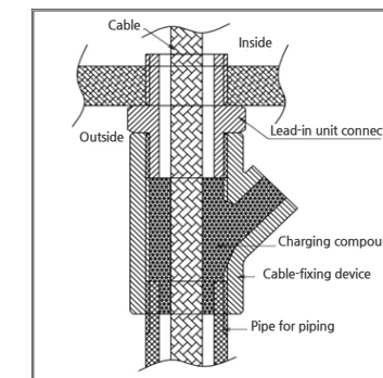
[Figure 12. Y Sealing Compound]
