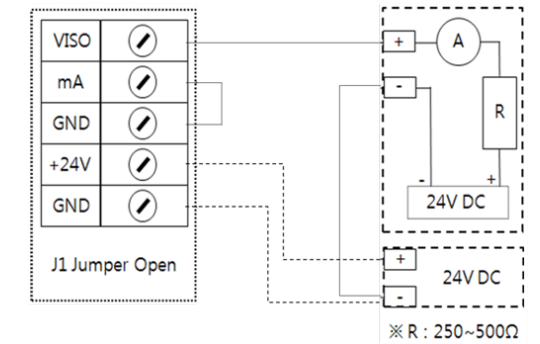
[Figure 7. 4~20mA 3 Wire Sink Driver Outline]
