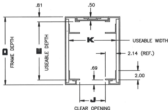
SECTION M-M
