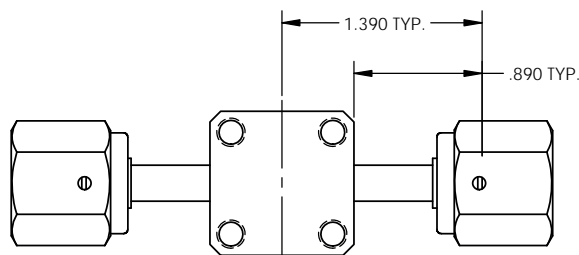
FEMALE FACE SEAL, SWIVEL
