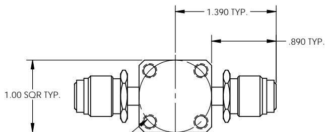
MALE FACE SEAL, SWIVEL
