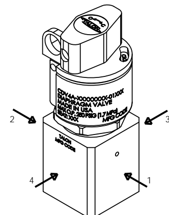
PORT CONFIGURATION DIAGRAM ORIENTATION AS SHOWN
