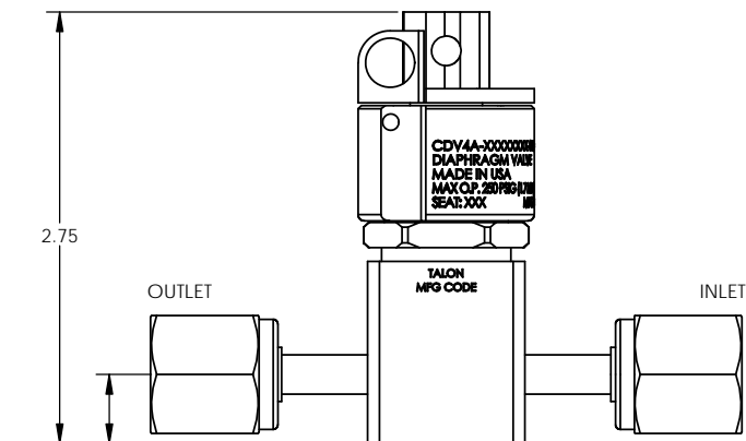
FEMALE FACE SEAL, SWIVEL A PORT CONFIGURATION
