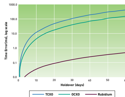
Accumulated Drift Error by Oscillator Type
